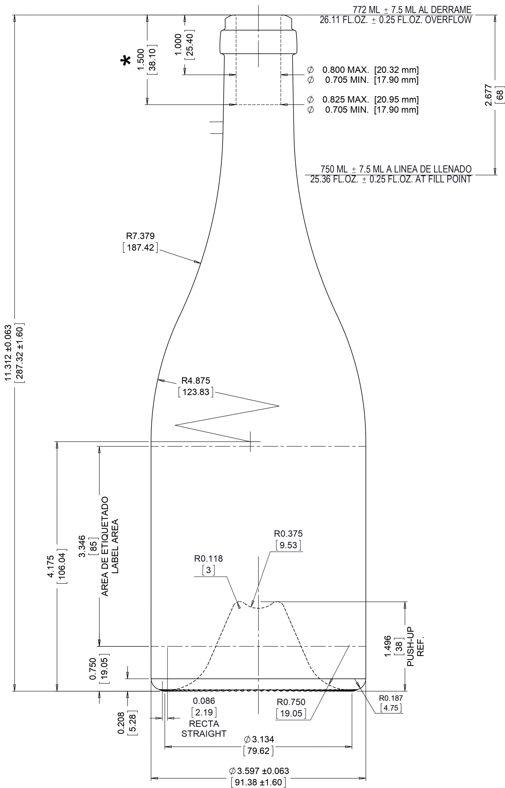
VISTA FRONTAL FRONT VIEW
